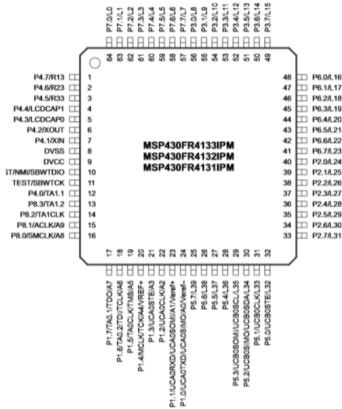
Figure 29: Pinout for MCU [27] (Image courtesy of Texas Instruments)
