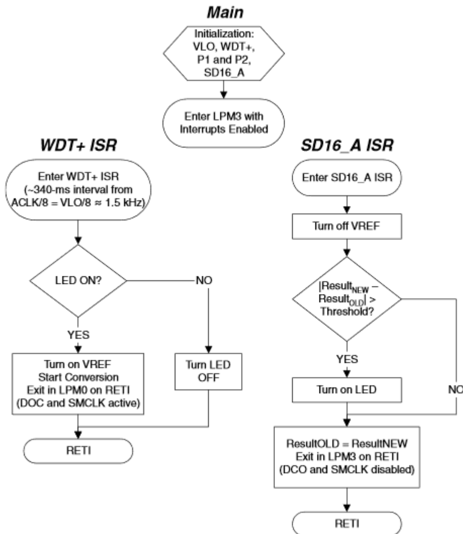
Figure 24: Motion Detection Software Flowchart [6] (Image courtesy of Texas Instrument)
