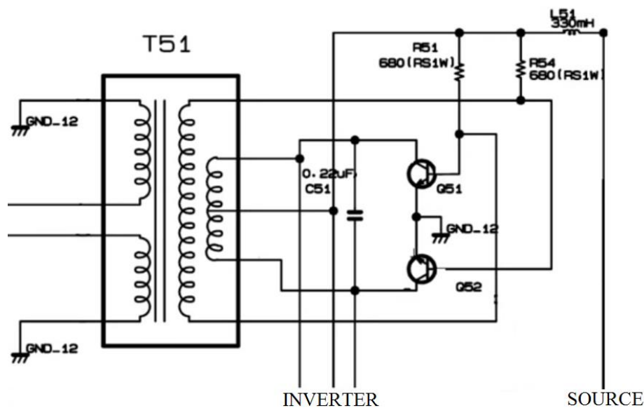
Figure 4: Diagram for a Simple Power Inverter [5]
