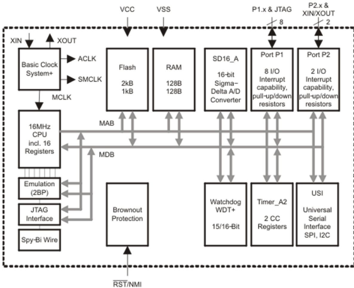
Figure 18: Functional Block Diagram for Microcontroller used in MSP430-PIR board, the MSP430F2013 [12] (Image Courtesy of Texas Instrument)
