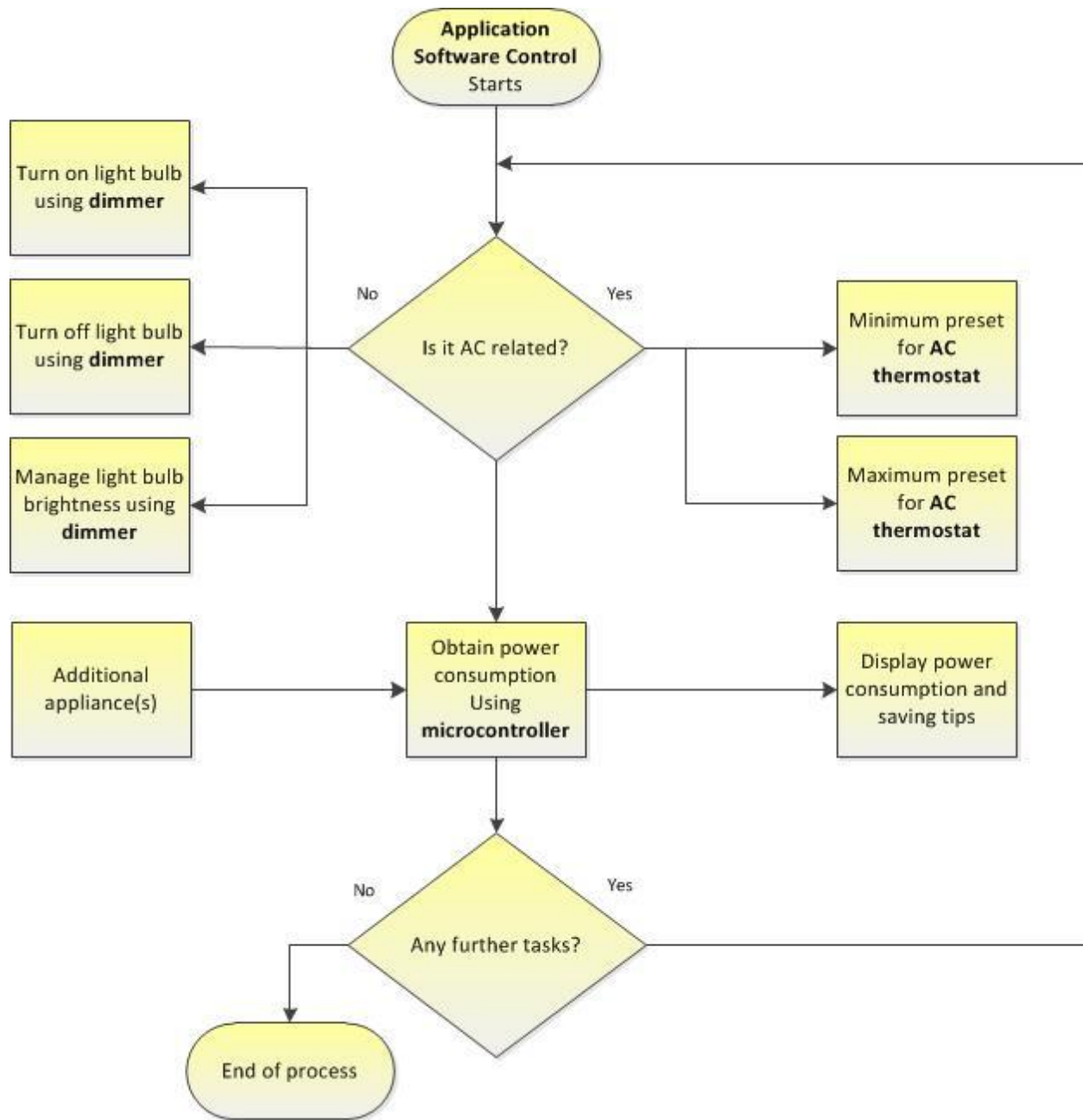
Figure 8: Application Software Control Process
