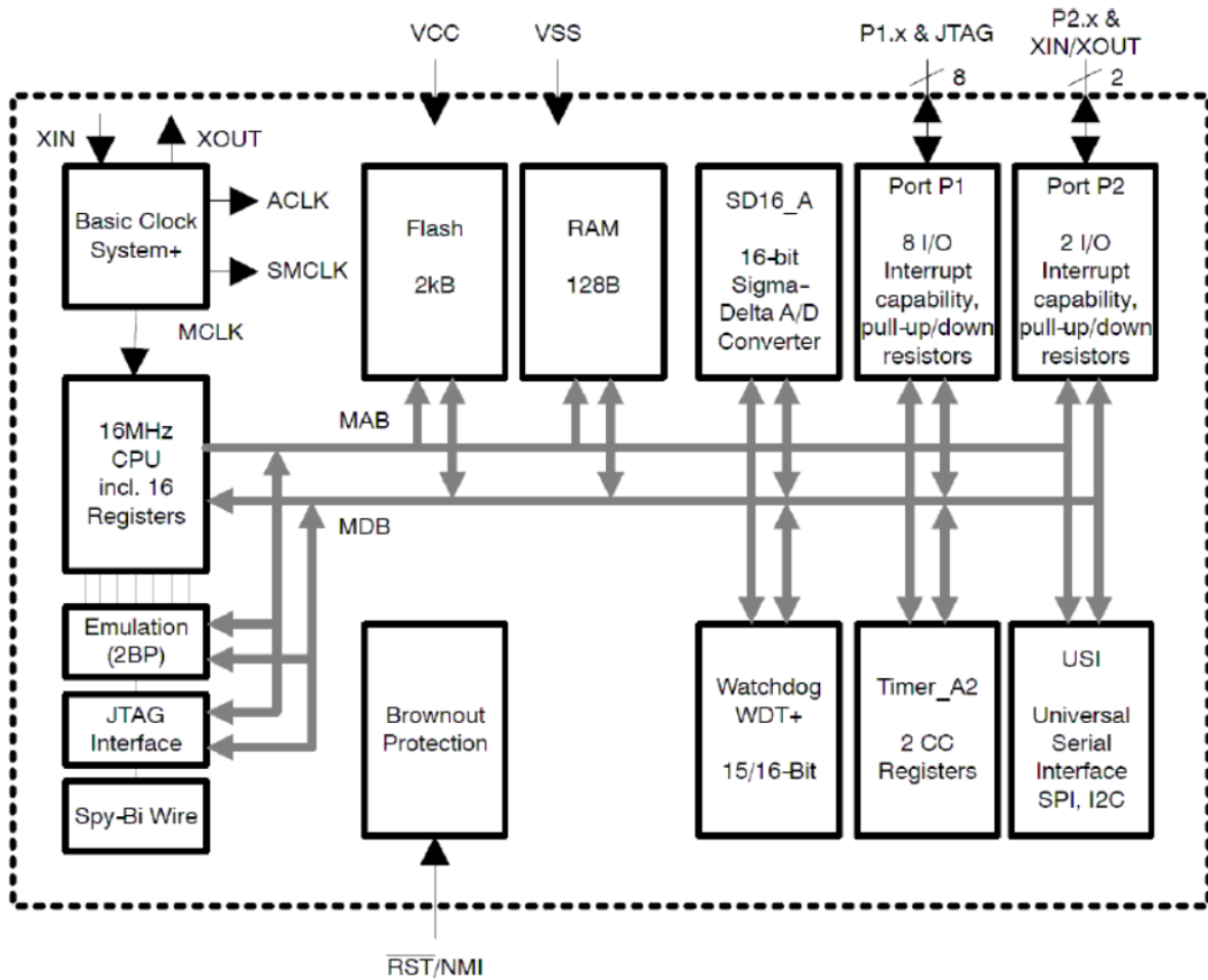
Figure 16: MSP430-PIR Sensor Block Diagram [4] (Image Courtesy of Texas Instruments)
