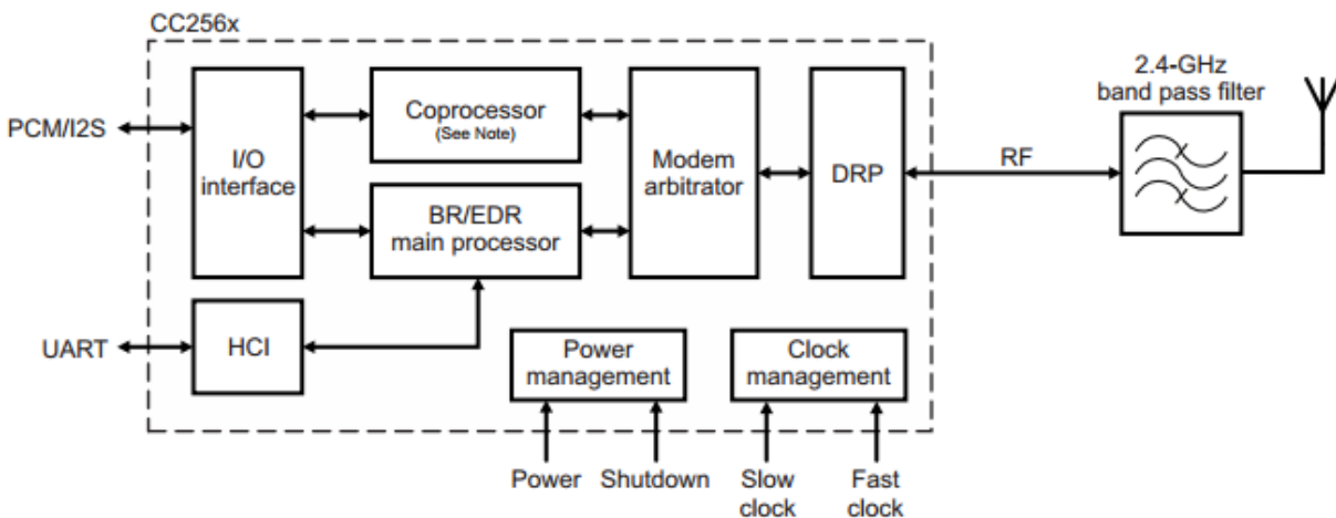
Figure 19: Functional Block Diagram of the Dual-Mode Bluetooth CC2564BRVMT [13] (Image Courtesy of Texas Instruments)
