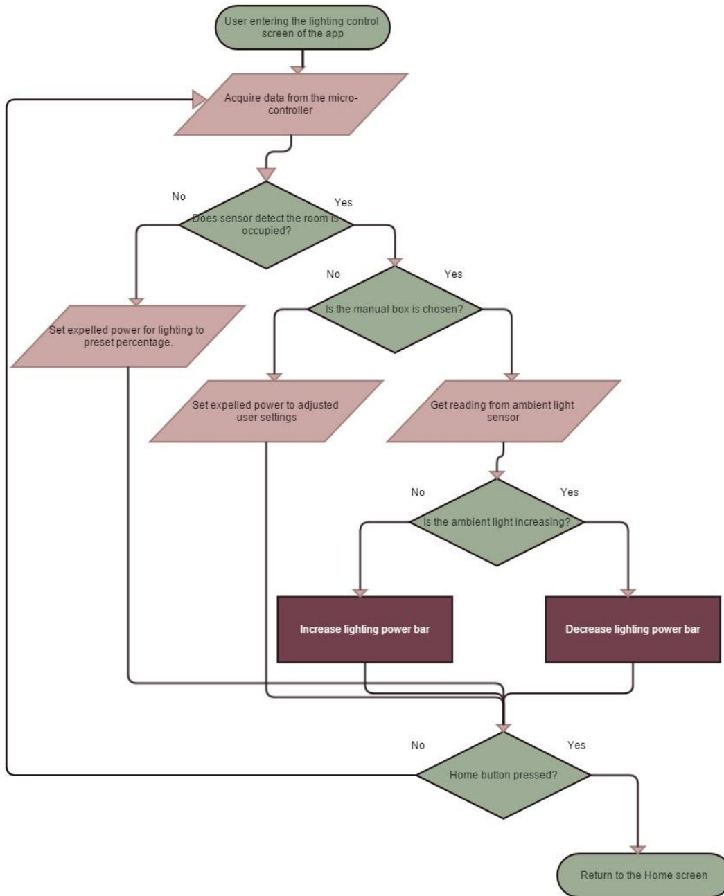
Figure 34: Lighting Control System Design Logic Flowchart
