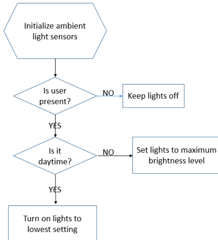
Figure 25: Dimmable Light System Characteristics Flowchart
