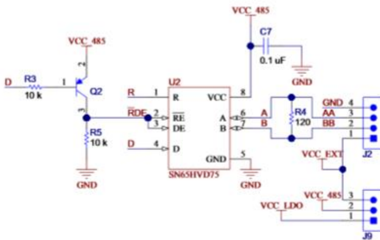
Figure 30: RS-485 Circuit (Image courtesy of Texas Instruments)
