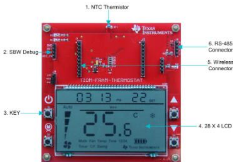
Figure 28: Basic AC Thermostat Board [27] (Image courtesy of Texas Instruments)
