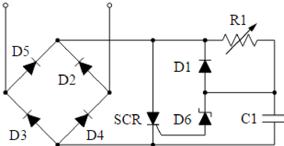
Figure 5: Diagram for a basic SCR Dimmer [6]
