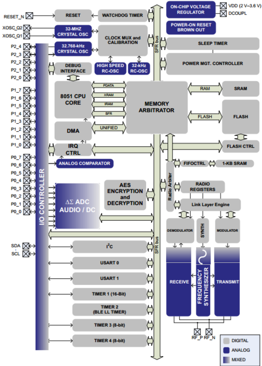
Figure 22: Block Diagram of the 2.4-GHz Bluetooth Low Energy and Proprietary SoC CC2541F256RHAR [18] (Image Courtesy of Texas Instruments)
