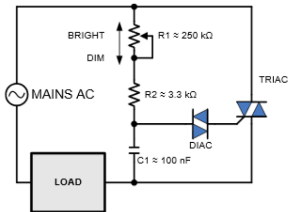
Figure 20: Simple Light Dimmer Circuit [16] (Image Courtesy of Texas Instruments)
