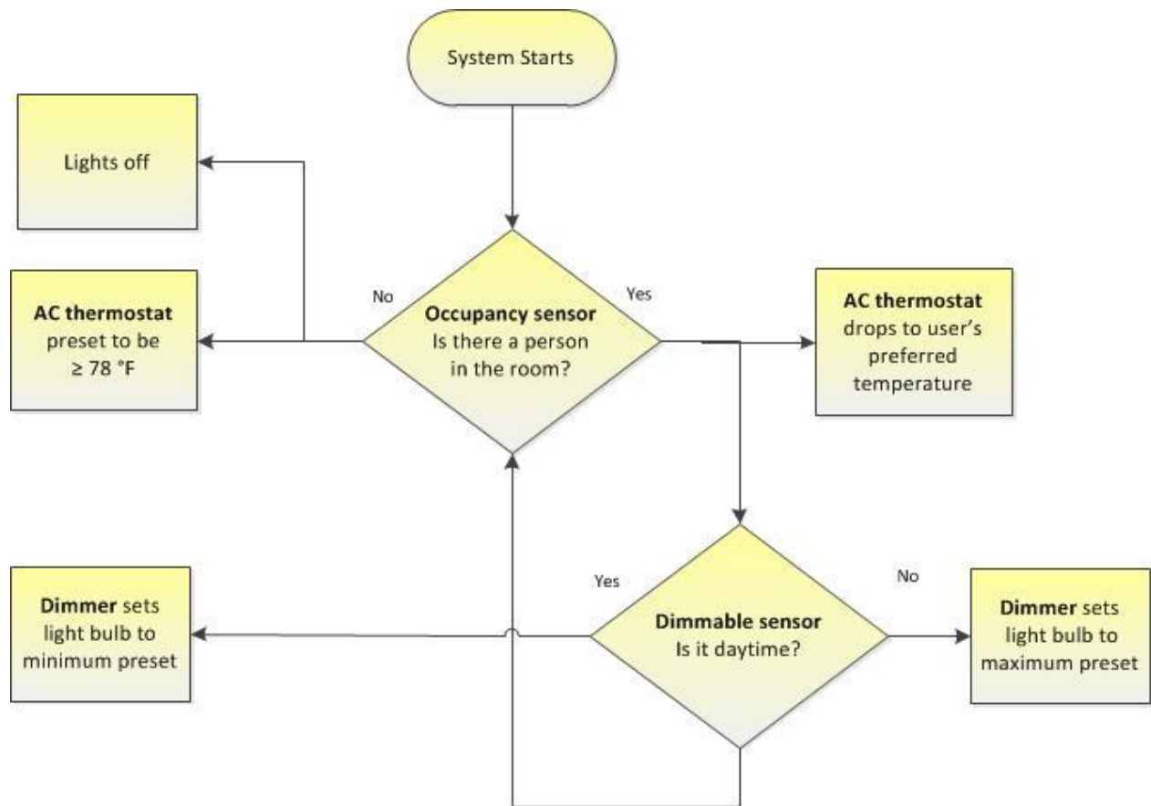
Figure 7: Occupancy & Ambient Light Sensor Process.
