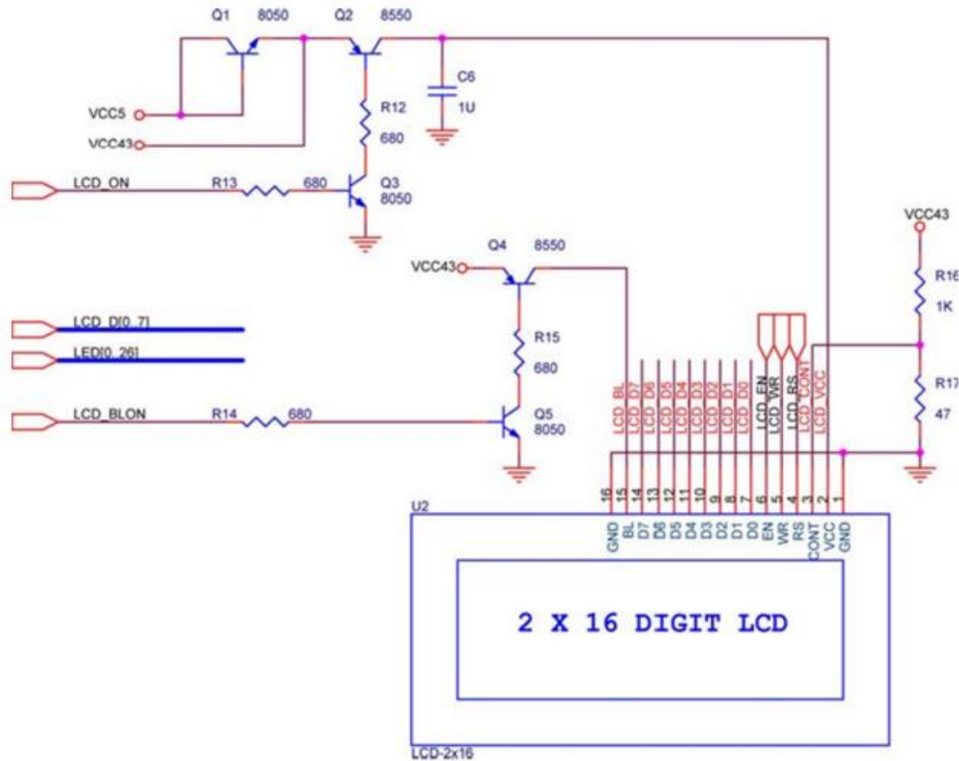
Figure 3: Diagram of a Simple LCD Module [4] (Reprinted with Permission of professor John S. Loomis from the University of Dayton)
