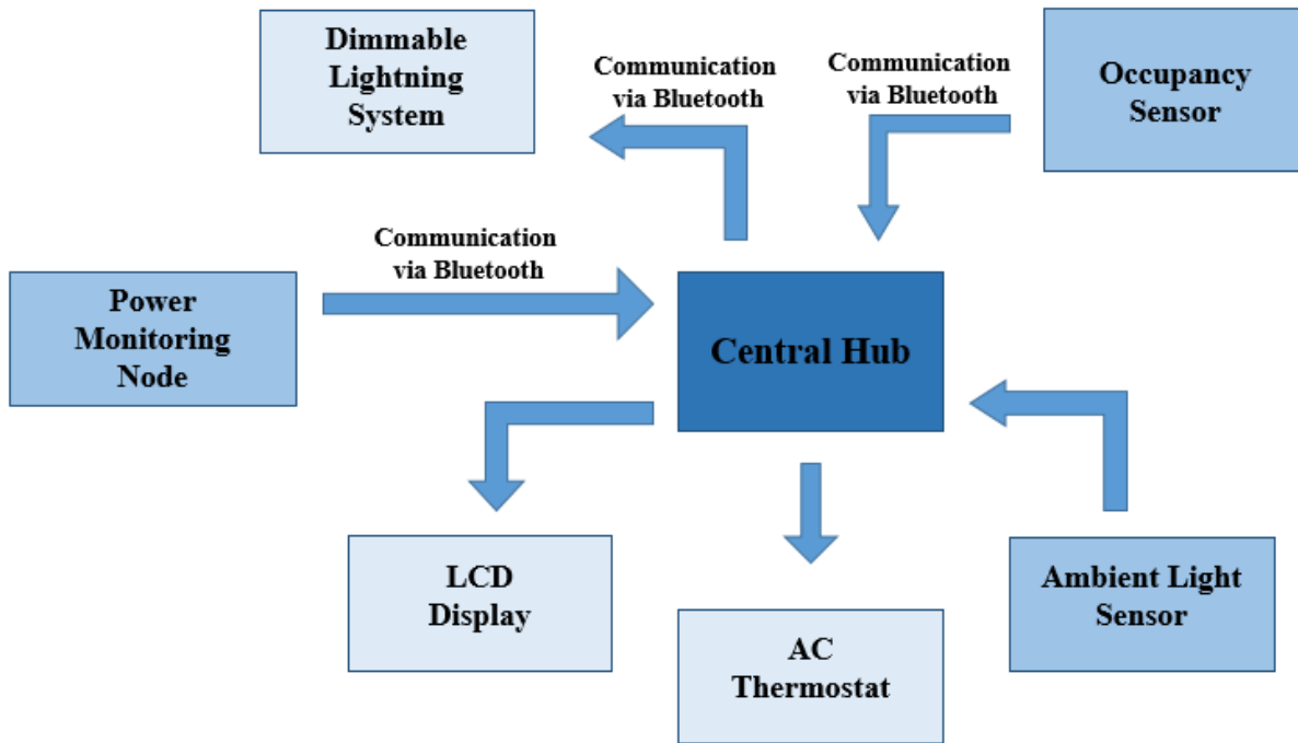
Figure 11: Diagram of Initial Hardware Diagram
