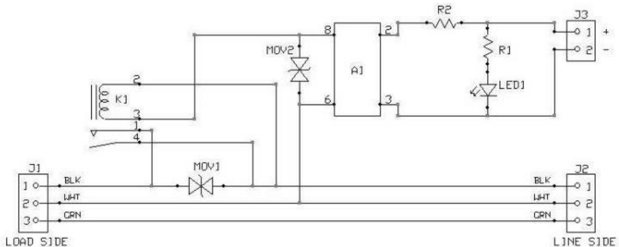
Figure 2: PowerSwitch Tail II circuit diagram [3] (Reprinted with Permission of the PowerSwitch Team)
