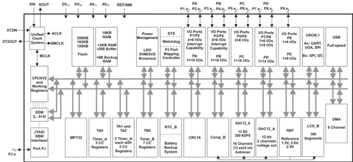
Figure 12: Functional Block Diagram for Microcontroller MSP430F6638 [8] (Image Courtesy of Texas Instrument)
