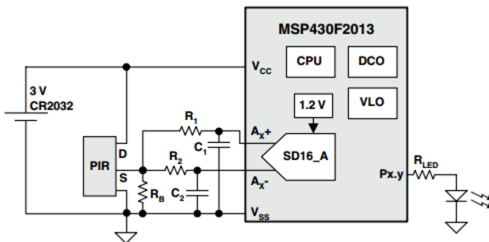
Figure 15: MSP430F2013 Motion Detection System [12]
